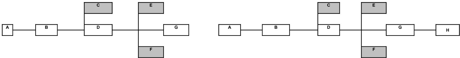
Existing System Modified System Typical single line diagram of a 33 KV Feeder
